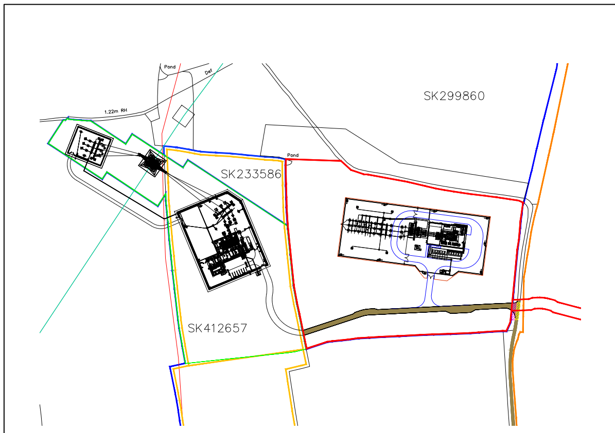
FIGURE 7: CONSENTED YAXLEY SUBSTATION
