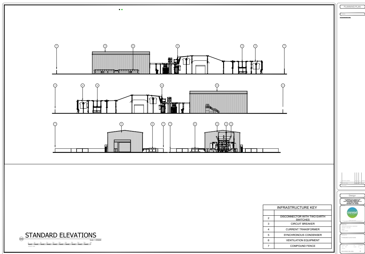
FIGURE 3: PLANNED DEVELOPMENT ELEVATIONS
