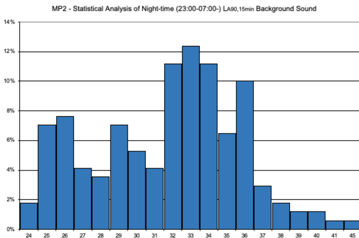
FIGURE 13: STATISTICAL ANALYSIS OF L_{A90} BACKGROUND – NIGHT-TIME – MP12
